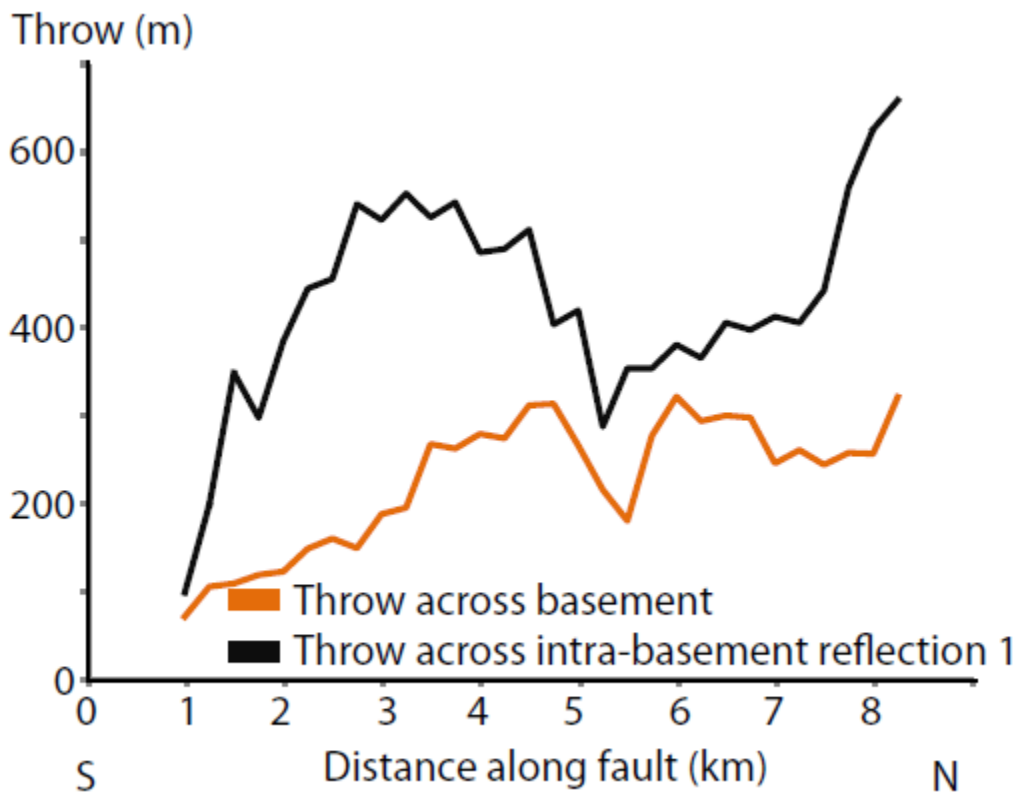
Figure S3. Throw vs. distance (T-x) plot for fault F1 at the structural levels of the basement reflection and intra-basement reflection 1 (see Fig. 1 for location of measurements).
