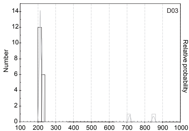
Fig. S1 Probability and weighted average of ^{206}\text{Pb}/^{238}\text{U} ages for representative sample D27, D28, D32, D56, D30, D36, and D03. Gray box in the probability diagram represents samples that plot outside of a Gaussian distribution, and they were excluded from the weighted mean age calculation. Gray bar in the weighted average plot represents the mean age.
