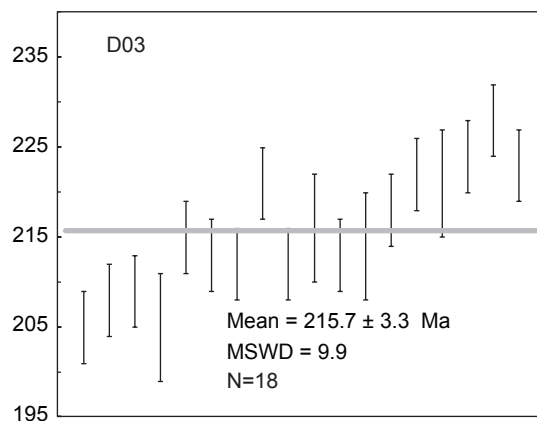
Fig. S1 Probability and weighted average of ^{206}\text{Pb}/^{238}\text{U} ages for representative sample D27, D28, D32, D56, D30, D36, and D03. Gray box in the probability diagram represents samples that plot outside of a Gaussian distribution, and they were excluded from the weighted mean age calculation. Gray bar in the weighted average plot represents the mean age.
