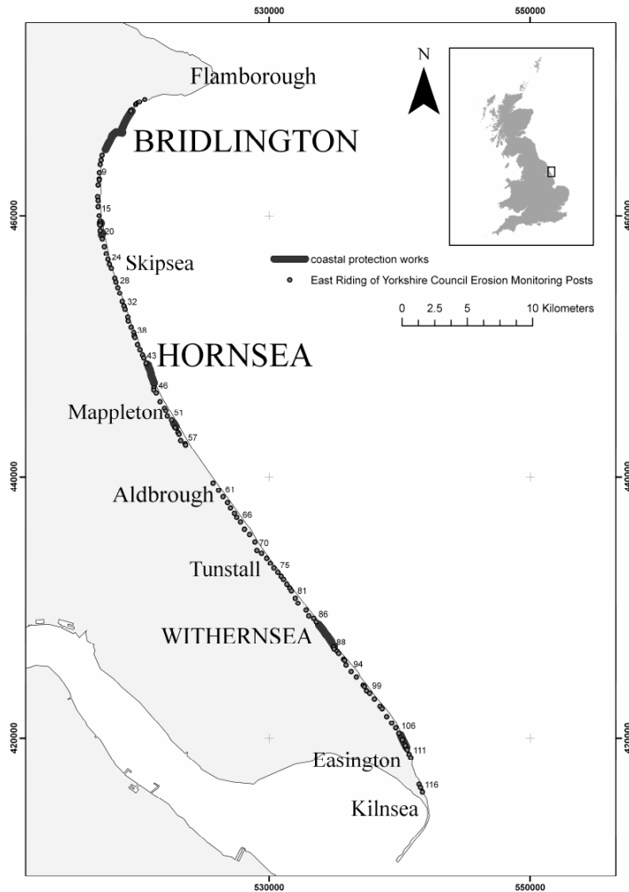
Location plan showing the position of Erosion Posts and coastal protection in relation to the Holderness coastline and the UK
